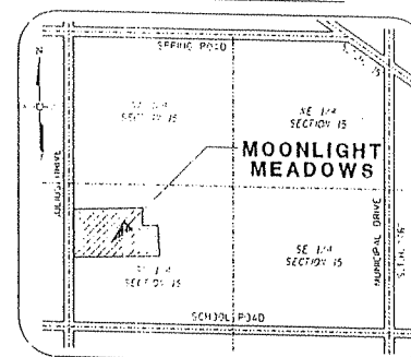
LOCATION MAP
